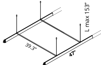
Joint detail 7KGTC/2-XX
