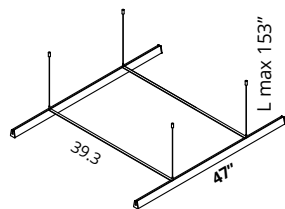
End Cap detail 7KTAP/4-XX
