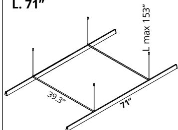
End Cap detail 7KTAP/4-XX
