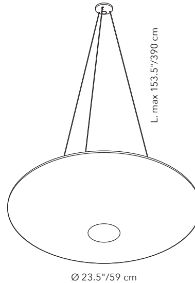
Chrome-plated ceiling plate
