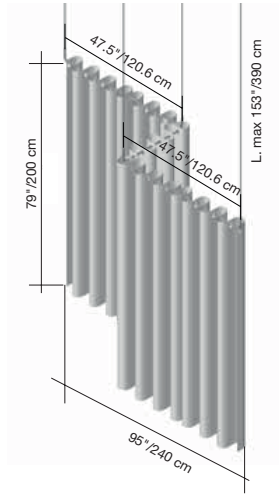
ITEM# 40041017: 4 ft (1.2 m) SUPPORT ROD (X2) ITEM# 40041016: 2 ft (.6 m) SUPPORT ROD (X1) ITEM# 40041015: END SUPPORTS (X2) ITEM# 40041014: CORNER SUPPORTS (X2) TEXTILE PANEL: (X5)
