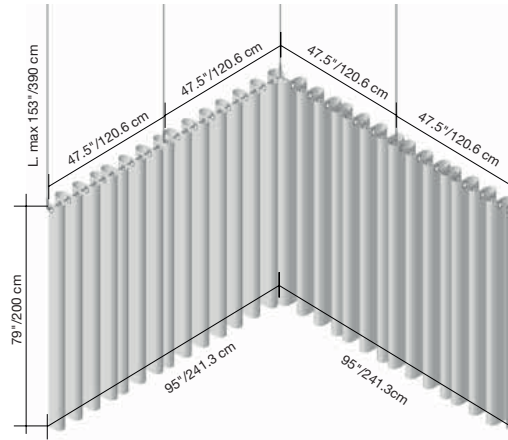
ITEM# 40041017: 4 ft (1.2 m) SUPPORT ROD (X4) ITEM# 40041015: END SUPPORTS (X2) ITEM# 40041014: CORNER SUPPORTS (X1) ITEM# 40041012: CENTRAL SUPPORTS (X2) TEXTILE PANEL: (X8)
