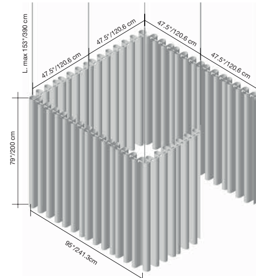
ITEM# 40041017: 4 ft (1.2 m) SUPPORT ROD (X7) ITEM# 40041015: END SUPPORTS (X2) ITEM# 40041014: CORNER SUPPORTS (X3) ITEM# 40041012: CENTRAL SUPPORTS (X3) TEXTILE PANEL: (X14)
